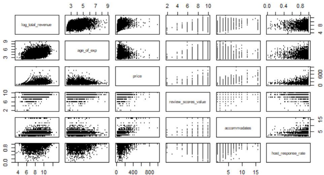
Scatterplot Matrix of AirBnB Variables against Log Total Revenue
