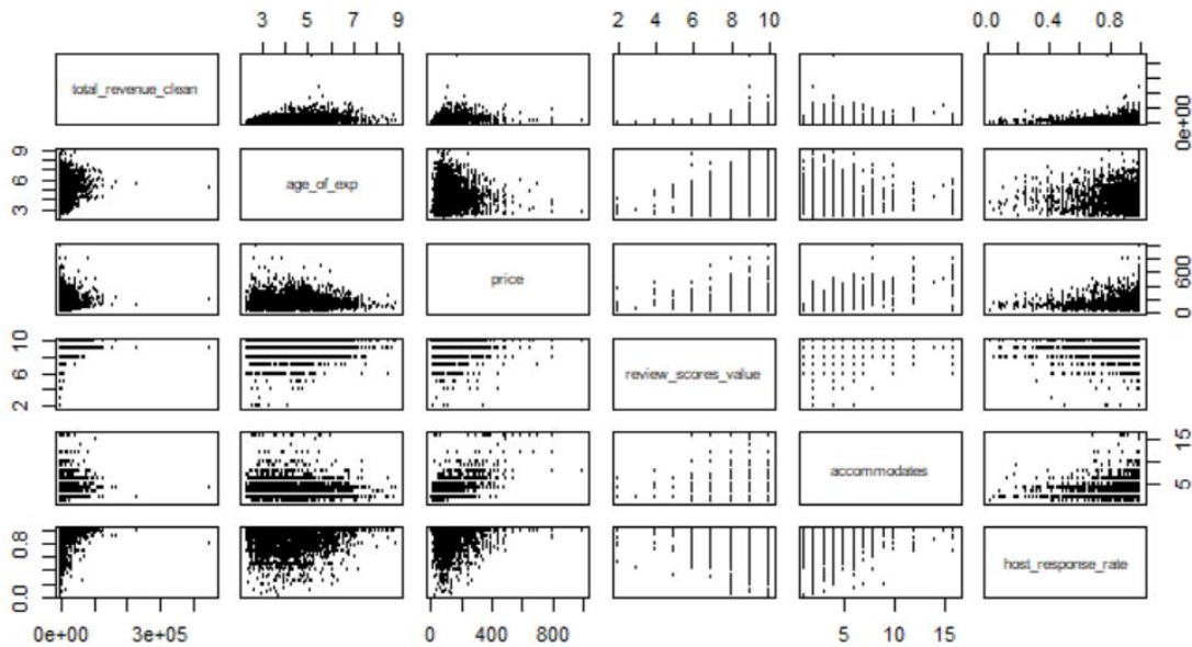
Scatterplot Matrix of AirBnB Predictors against Total Revenue
